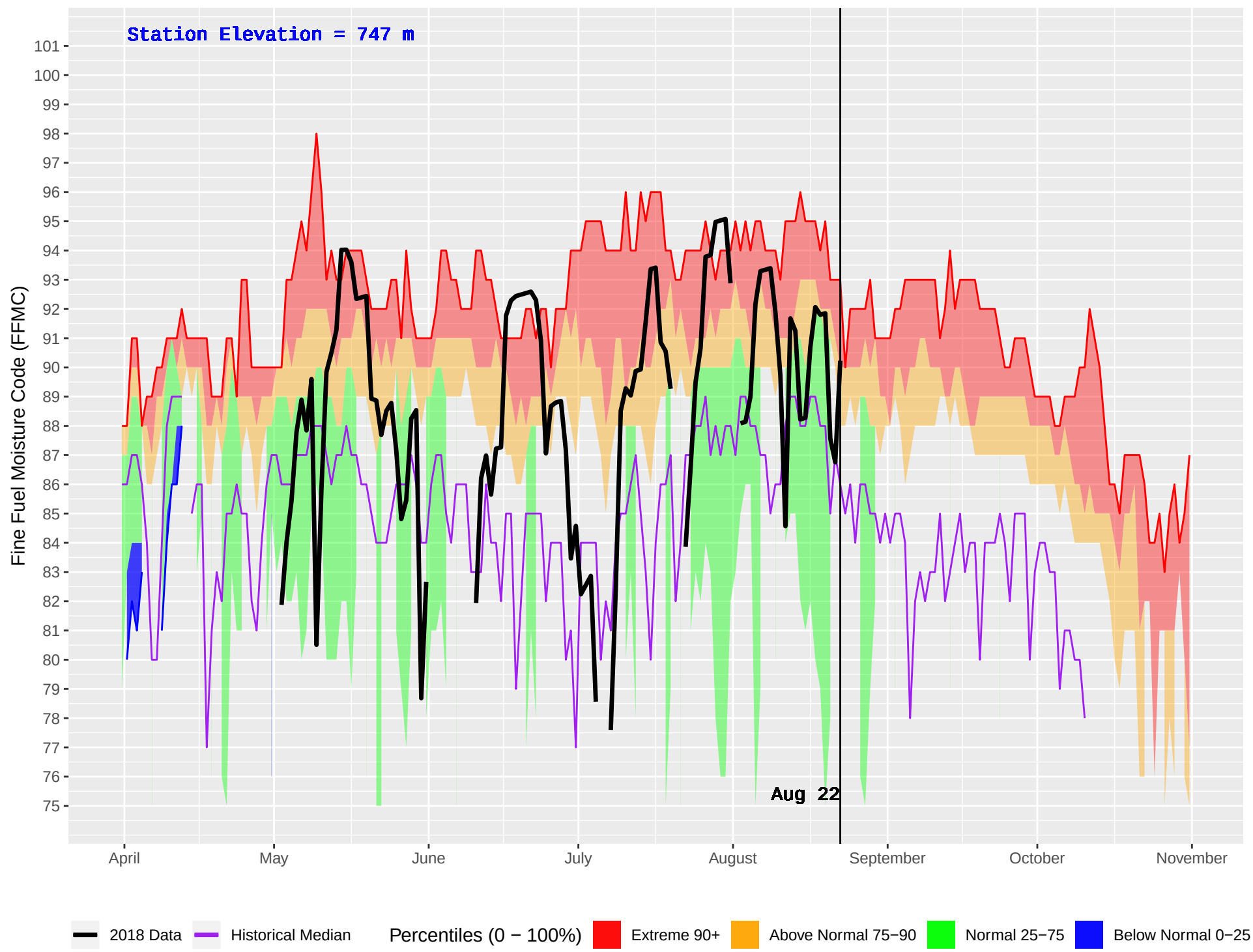
PEDEN (178) : Historical (1984–2016) and Current (2018) Daily Fine Fuel Moisture Code (FFMC)
